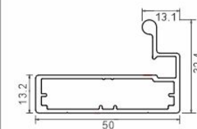
AVAP 1031 Aluminium Profile With Handle Size : 3000mm
