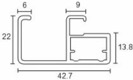
AVAP 045 Aluminium Profile With Handle Size : 3000mm
