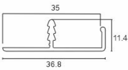
AVAP 053 Aluminium Edge Profile Size : 3000mm
