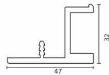
AVAP 1096 Aluminium Handle Profile Size : 3000mm
