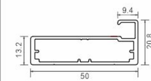
AVAP 1005 Aluminium Profile Size : 3000mm
