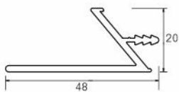
AVAP 1076 Aluminium Handle Profile Size : 3000mm
