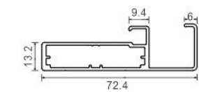
AVAP 094 Aluminium Profile With Handle Size : 3000mm
