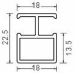
AVAP 076 I Aluminium 'I' Profile For 6mm Glass Size : 3000mm
