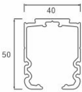
AVSC 027 Aluminum Profile Size 3660mm (12)
