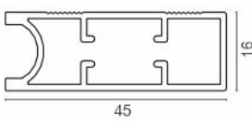
AVAP 1050 Aluminium Profile Size : 3000mm
