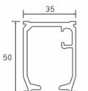
AVSC 402 ₹ 8300.00 /- PCS Aluminum Profile for AVSLD 402 Finish : ALU Size : 3660mm (12)
