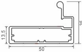
AVAP 1031 A Aluminium Profile with Handle For 6mm Glass Size : 3000mm
