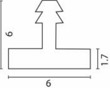
AVAP 1078 Aluminium Inlay Profile Size : 3000mm
