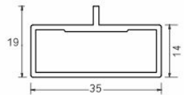
AVAP 1097 Aluminium Profile Size : 3000mm
