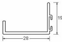
AVAP 1090 Aluminium Handle Profile Size : 3000mm
