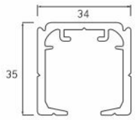
AVSC 028 ₹ 5600.00 /- PCS Aluminum Profile for AVSLD 028 Finish : ALU Size 3660mm (12)
