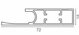
AVAP 1051 Aluminium Handle Profile Size : 3000mm
