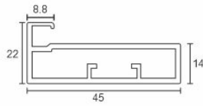
AVAP 1004 Aluminium Profile Size : 3000mm
