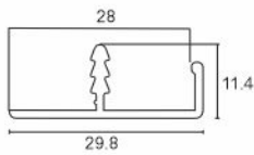
AVAP 052 Aluminium Edge Profile Size : 3000mm
